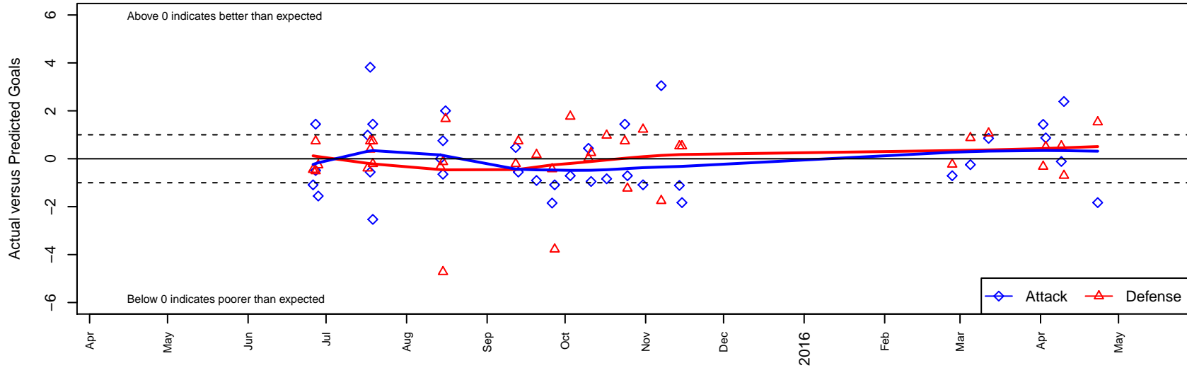
HSC Real G04 Dots are actual minus expected GF (blue circles) and GA (red triangles). Blue line is smoothed change in attack strength. Red is smoothed change in defense strength.
